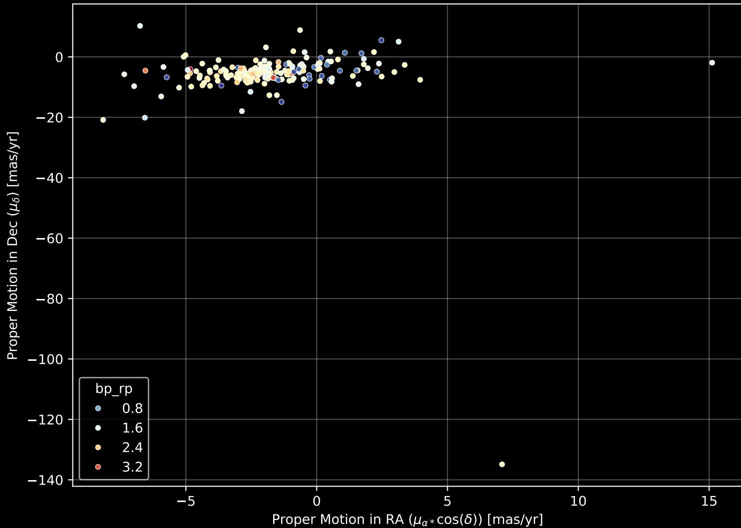
APOGEE DR17 Field: [045+06] Proper Motion Diagram (n= 195)
