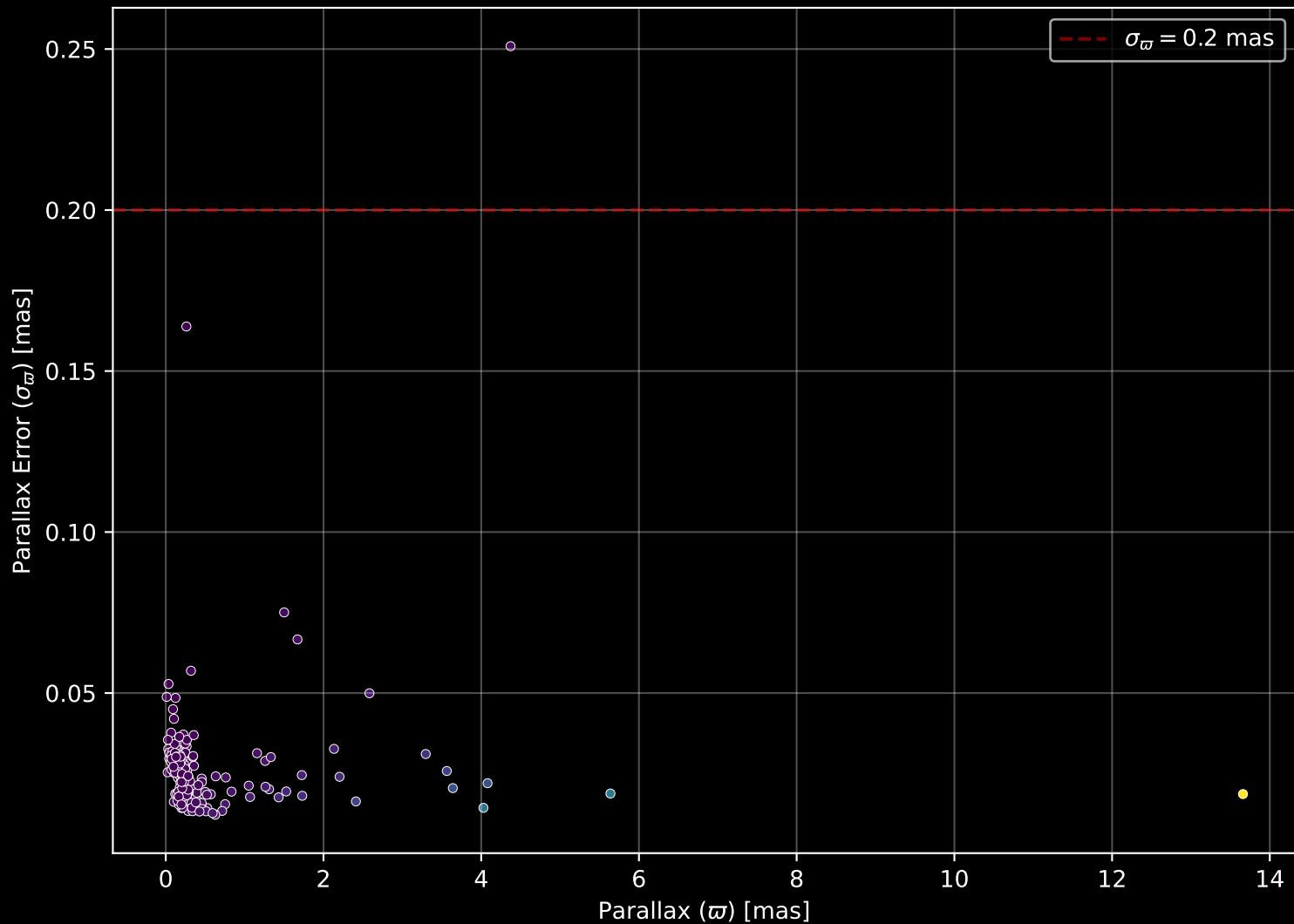
APOGEE DR17 Field: [045+06] Parallax Quality (n= 195)
