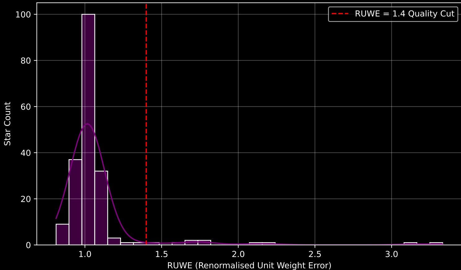
GAPOGEE DR17 Field [045+06] RUWE Distribution (n= 193)
