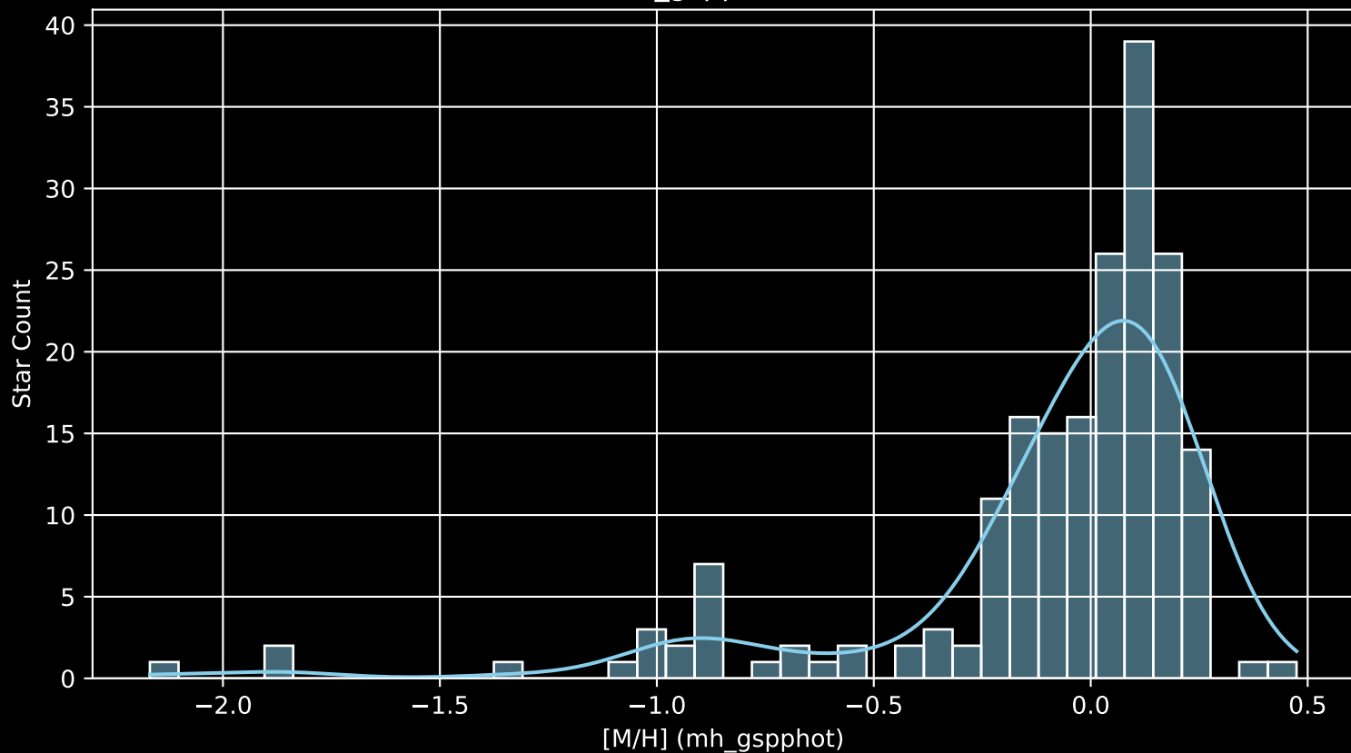
APOGEE DR17 Field: [045+06 [M/H] (mh_gspphot) (n= 195)
