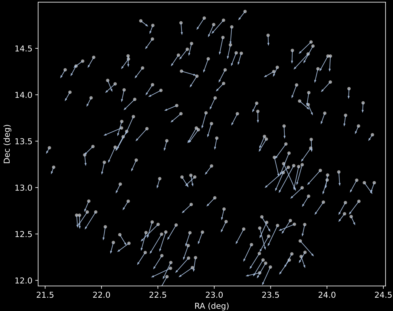
APOGEE DR17 Cluster 1 Proper Motion Vectors (n=167)
