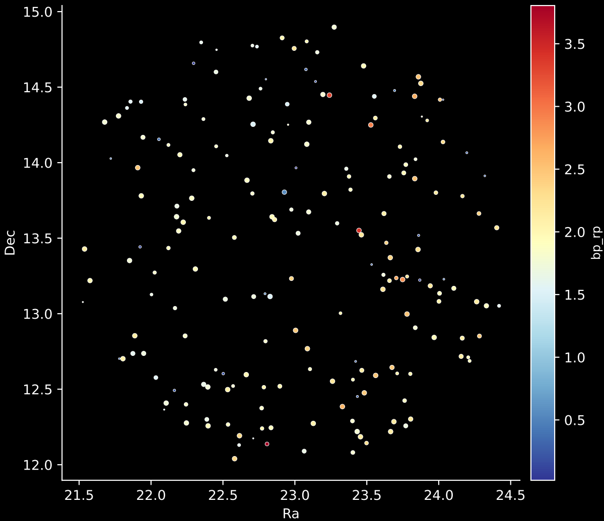
APOGEE DR17 Field: [045+06] Stars: 195
